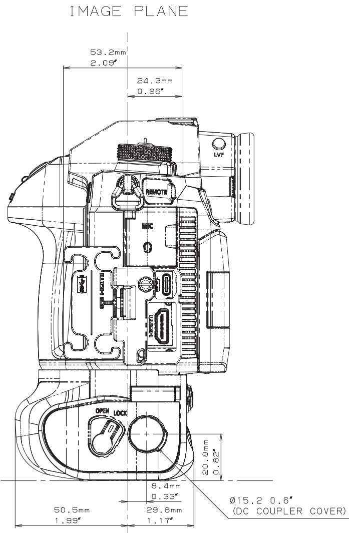
CAMERA LEFT
