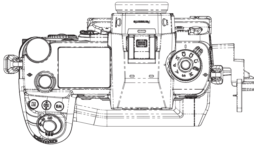
CAMERA TOP
