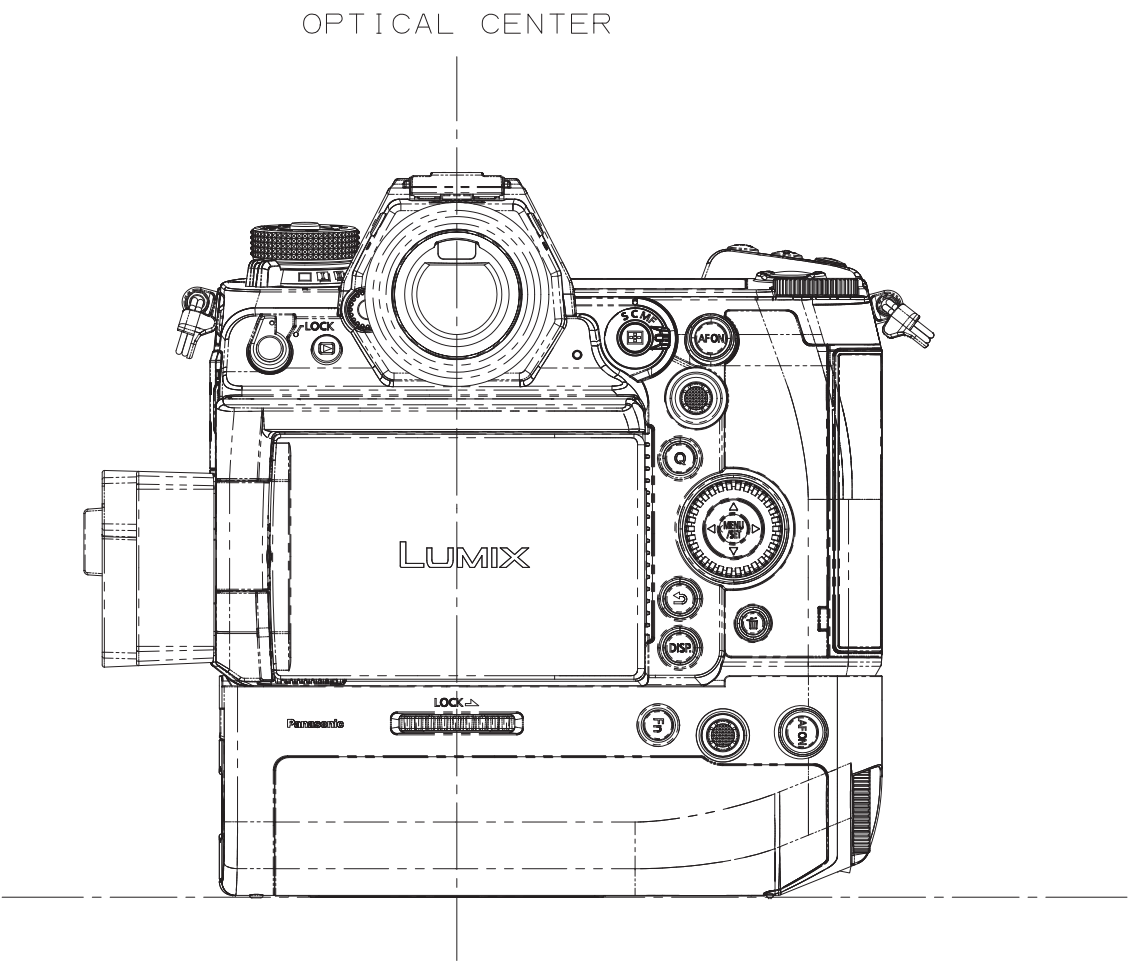
CAMERA BACK
